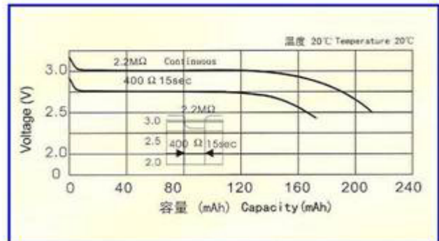
脉冲放电曲线 Pulse Discharge Characteristics
